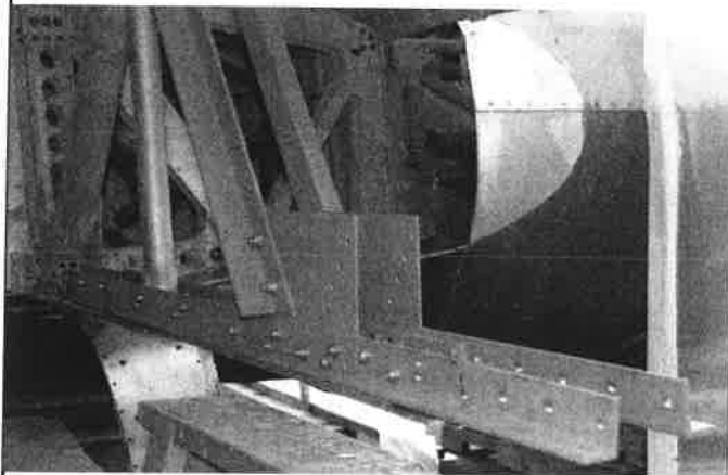
The reconstructed Hampden wing spar and fittings. Note the original metal of the engine nacelle in the background, showing the corrosive effects of 30 years on the sea bed.
